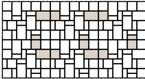
Pattern B - Stack Bond
